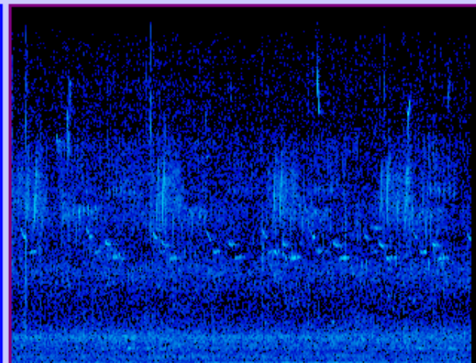
Spectrogram
